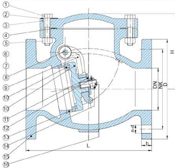
DIMENSIONS IN INCHES AND MILLIMETRES
